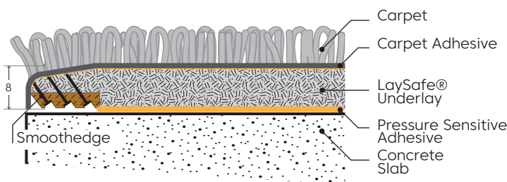
Stretch Fit Installation Section
